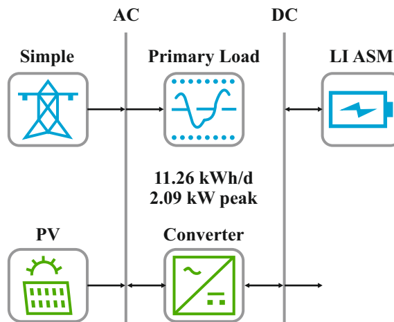
Figure 3: Design Diagram of Solar Powered Villages
